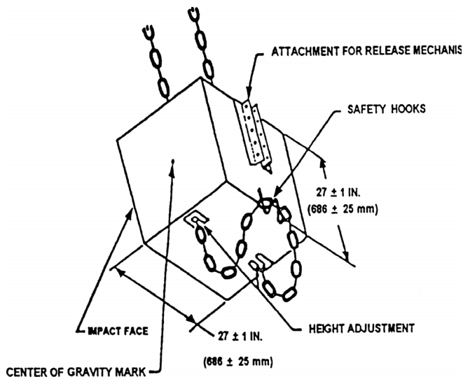
FIGURE V-22 Pendulum.
