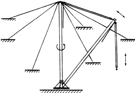
Guyed Derrick
