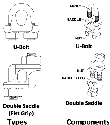
Figure 35 Wire Rope Clips
