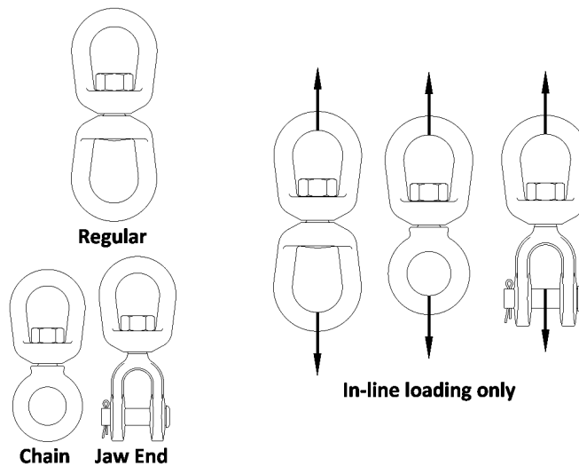
Figure 38 Swivels
