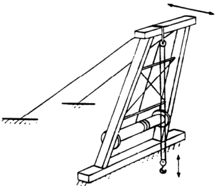
Breast Derrick
