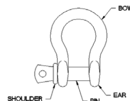
Figure 27 Typical Shackle Components
