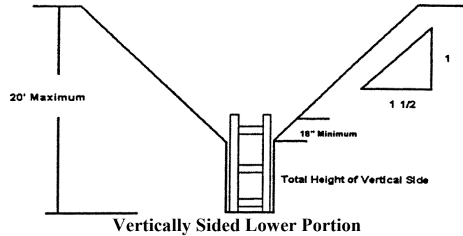
Figure N-12 Slope Configurations for Type C Soil Support or Shield System
