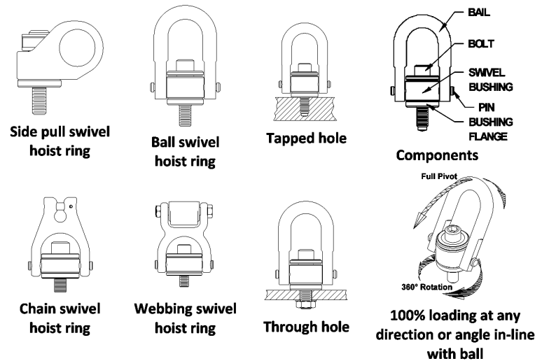
Figure 34 Swivel Hoist Rings
