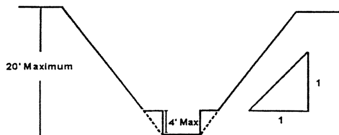
Figure N-8 Slope Configurations for Type B Soil This bench allowed in cohesive soil only.
