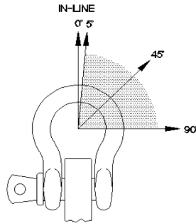
Figure 28 Side Loading
