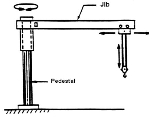
Pedestal-Jib Crane
