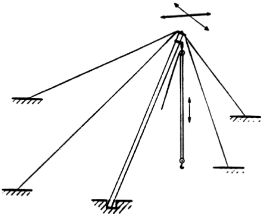
Gin-Pole Derrick
