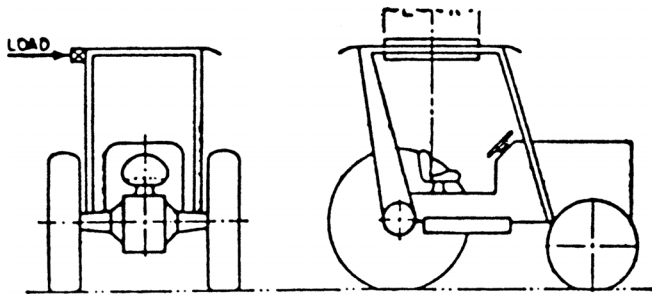
FIGURE V-25 Location for side load.
