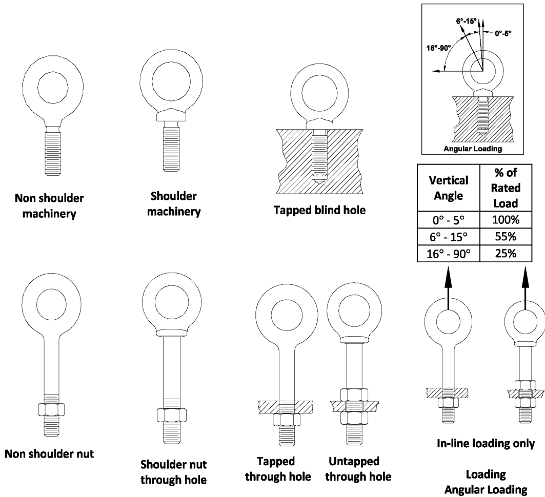
Figure 31 Eyebolts
