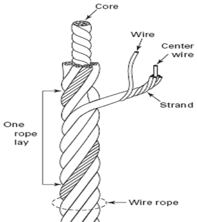
Figure 1 - Wire Rope
