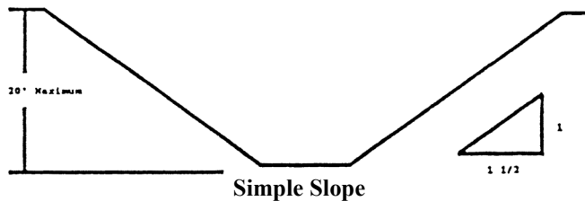
Figure N-11 Simple Configurations for Type C Soil
