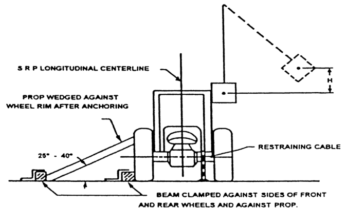
FIGURE V-24 Method of impact from side.
