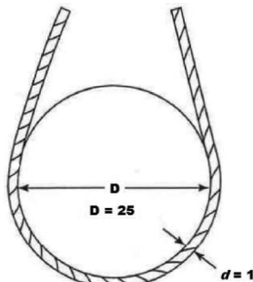
Figure 19 D/d Ratio
