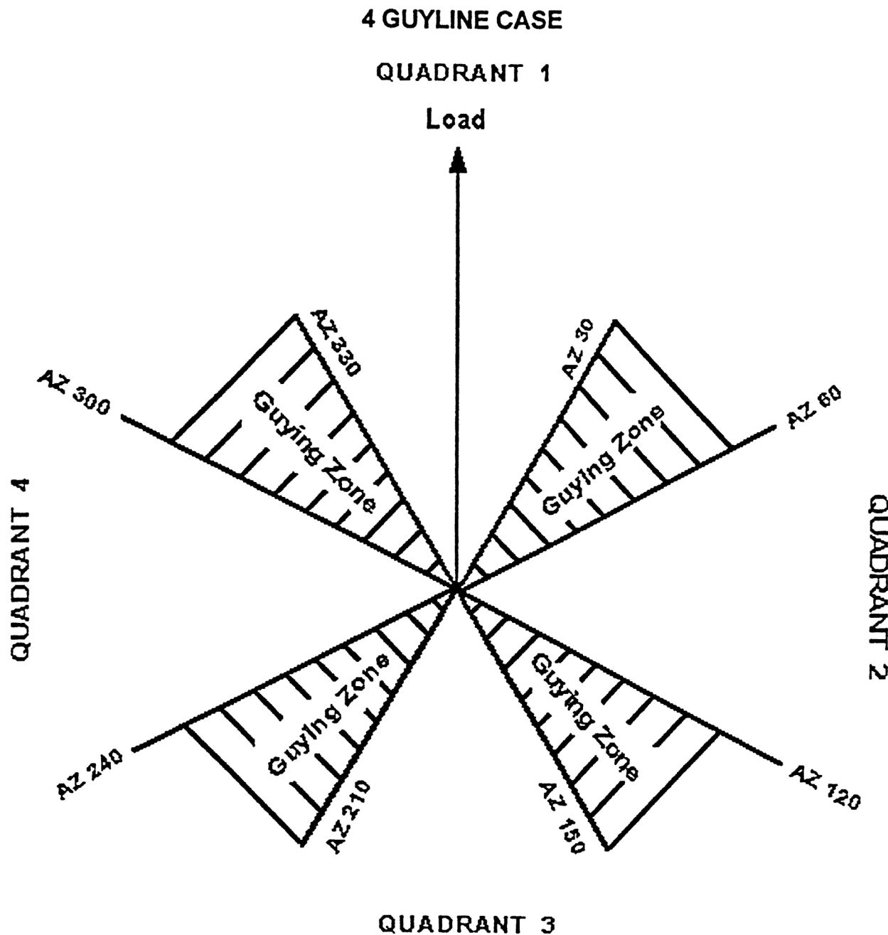
Figure 8: 4 Guyline Case
