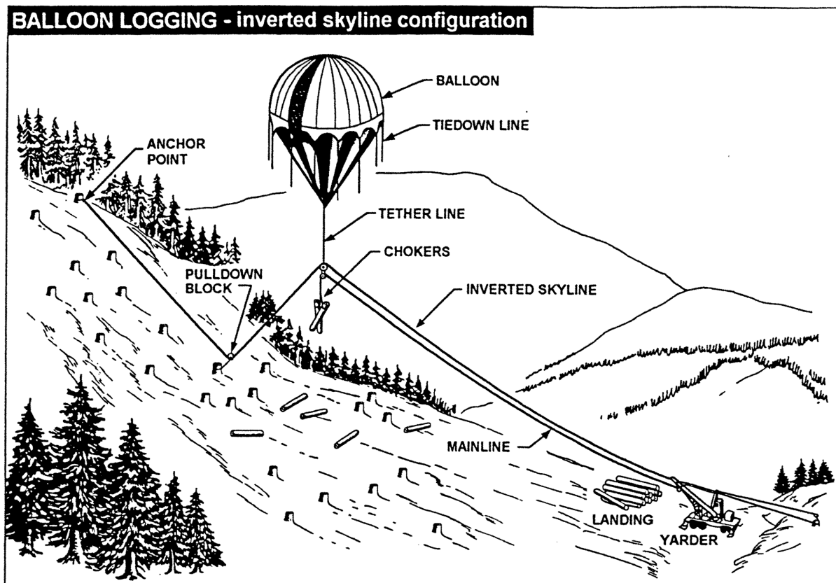
Figure 57: Balloon Logging - Inverted Skyline Configuration
