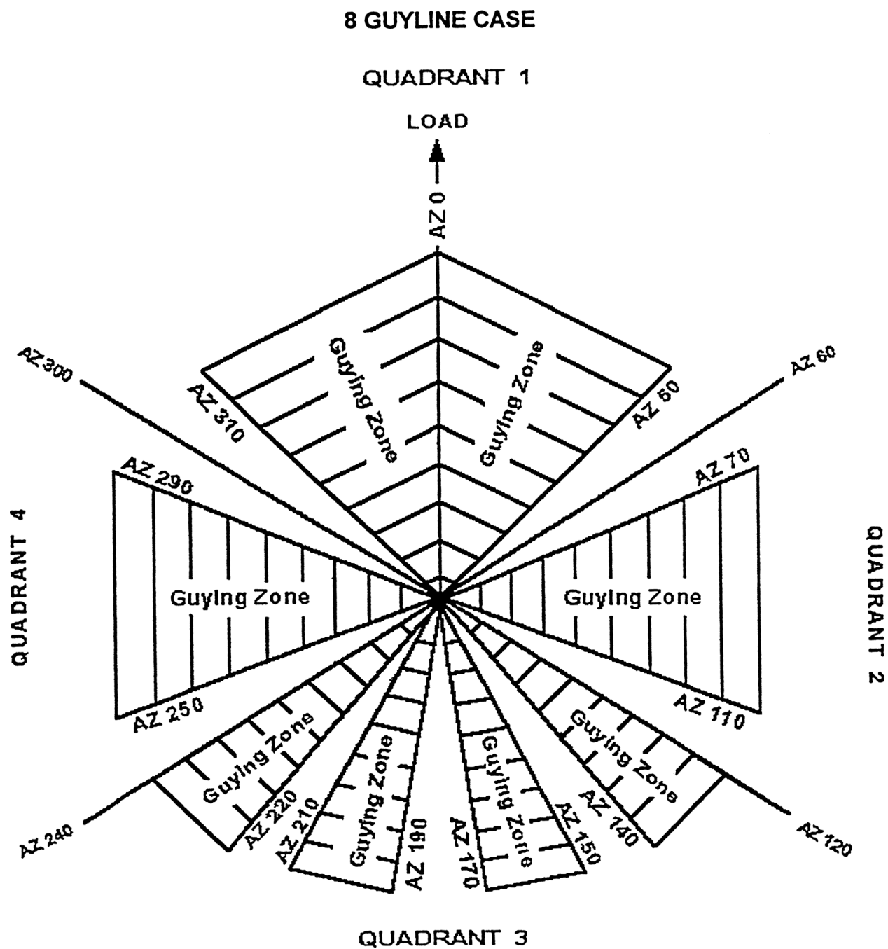
Figure 15: 8 Guyline Case (2)
