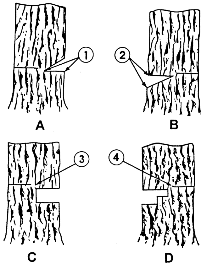
FIGURE 2: UNDERCUTS
