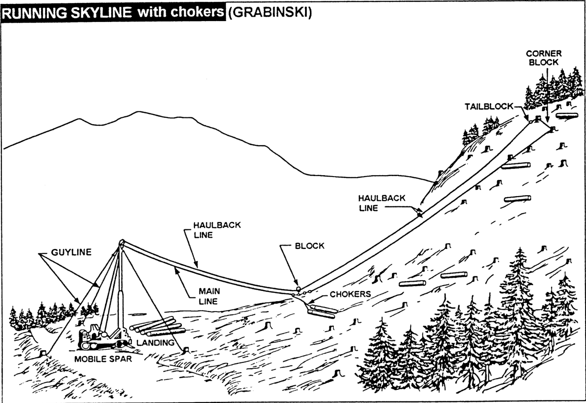
Figure 54: Running Skyline with Chokers (Grabinski)
