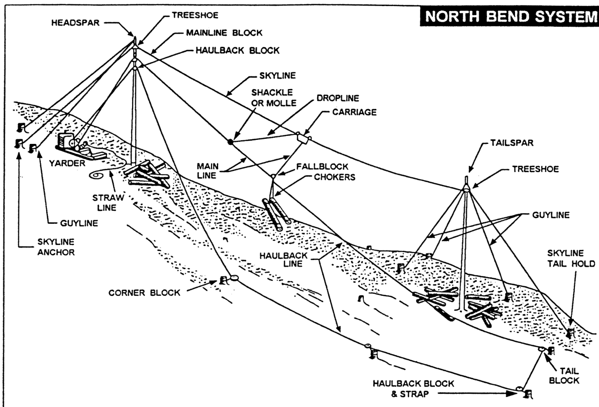
Figure 49: North Bend System
