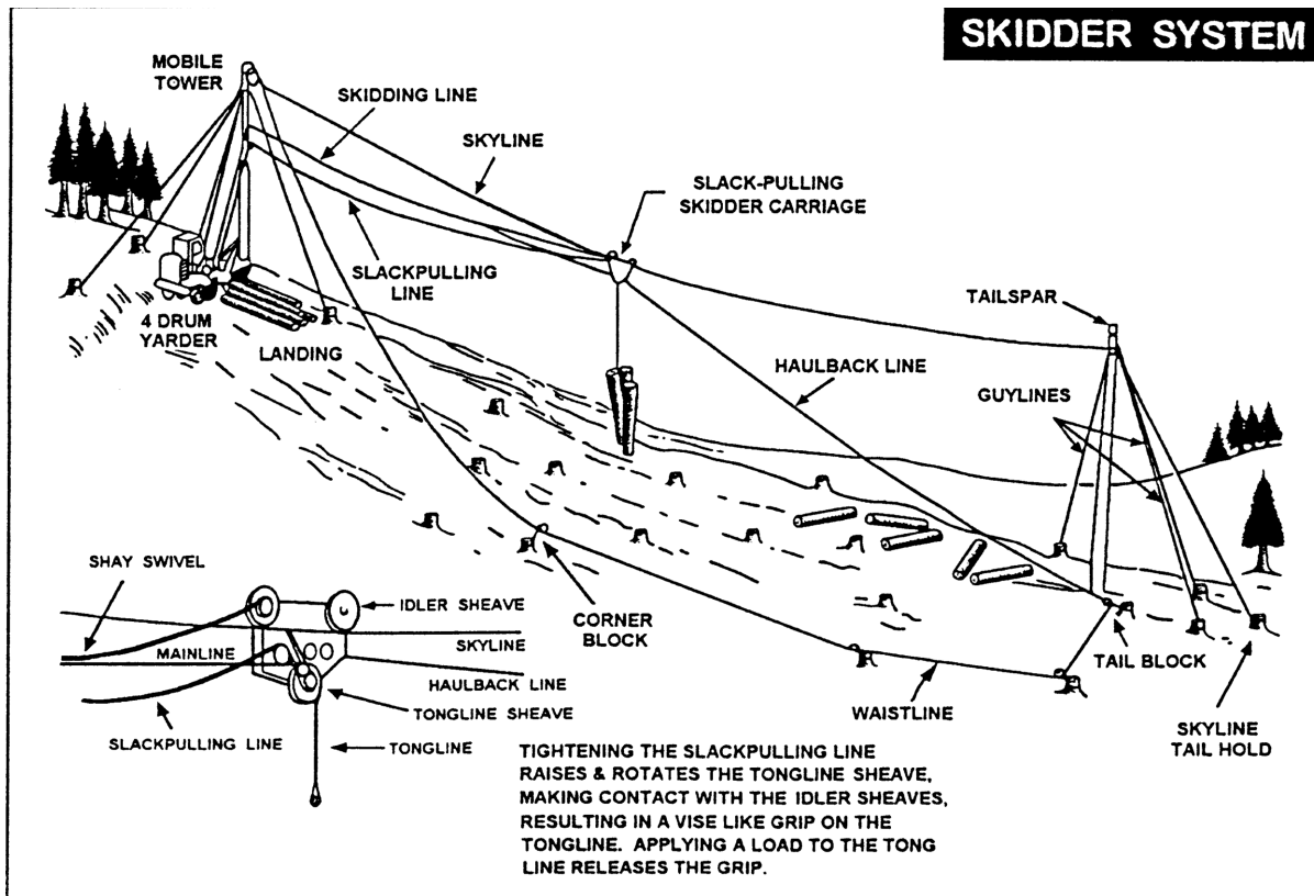
Figure 48: Skidder System
