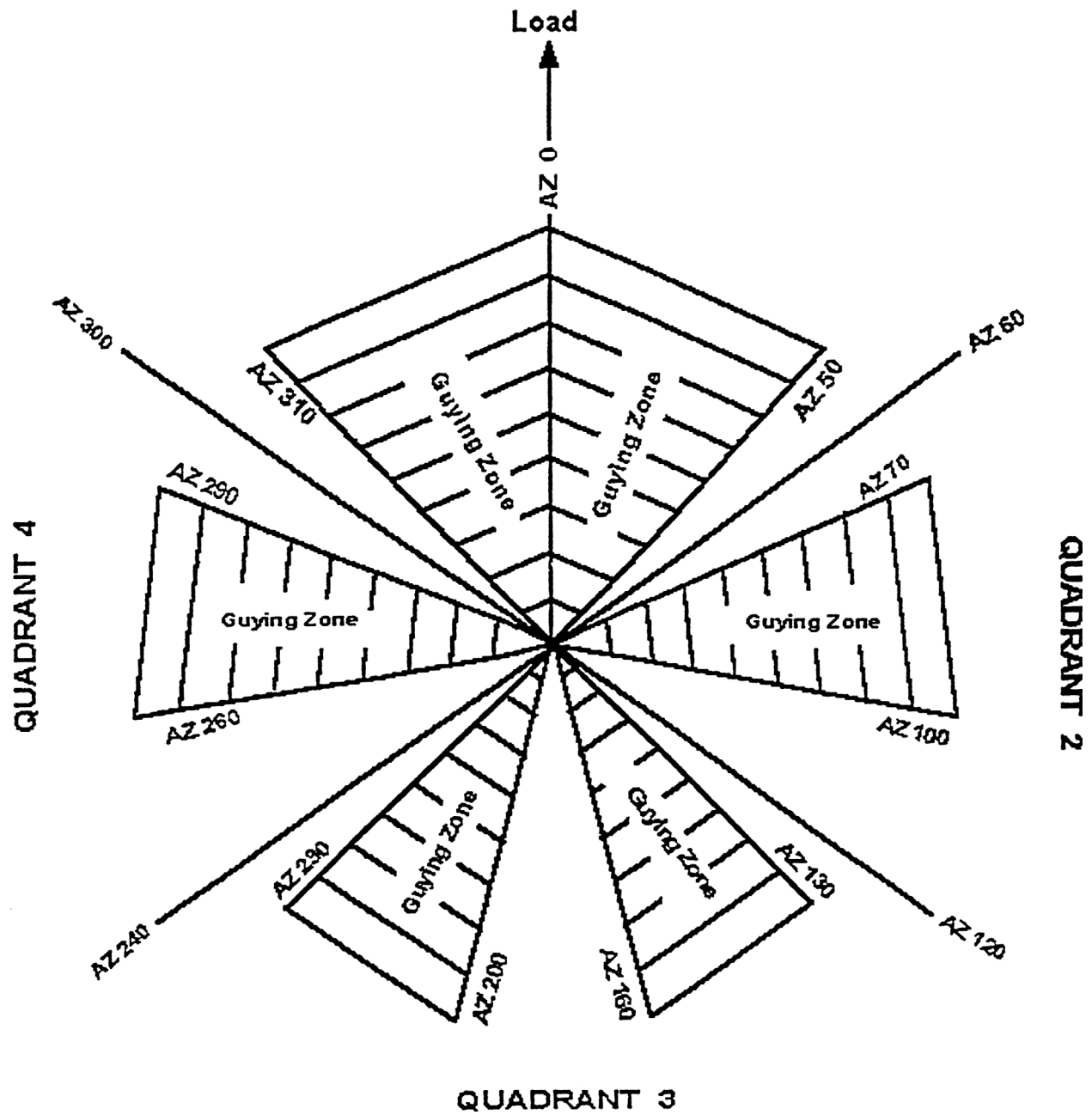
Figure 11: 6 Guyline Case
