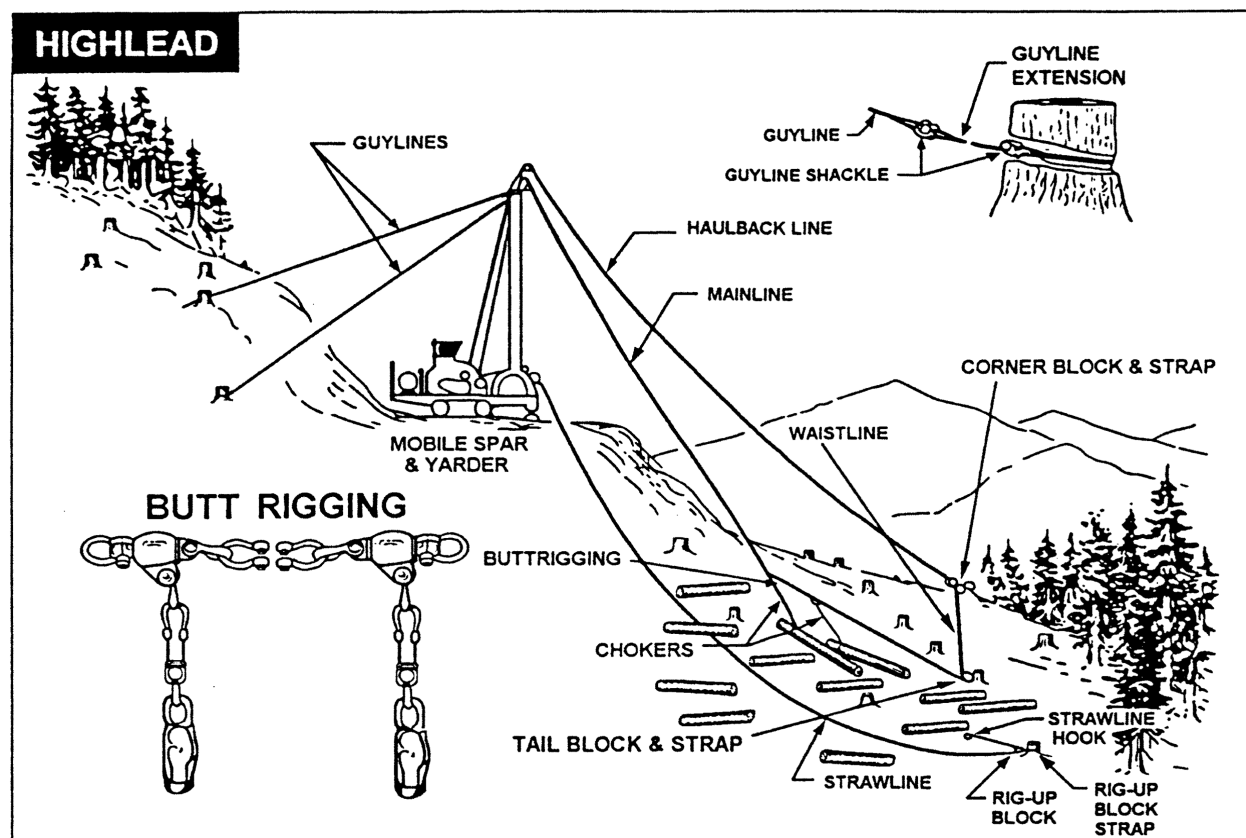
Figure 45: Highlead
