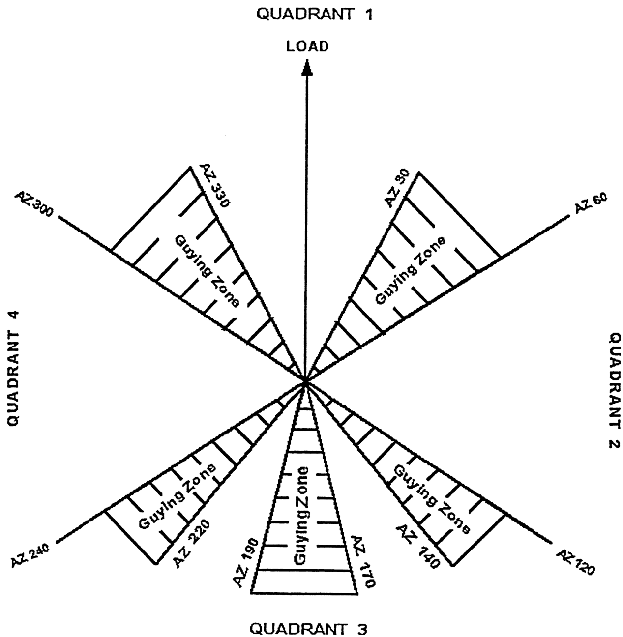
Figure 10: 5 Guyline Case (2)
