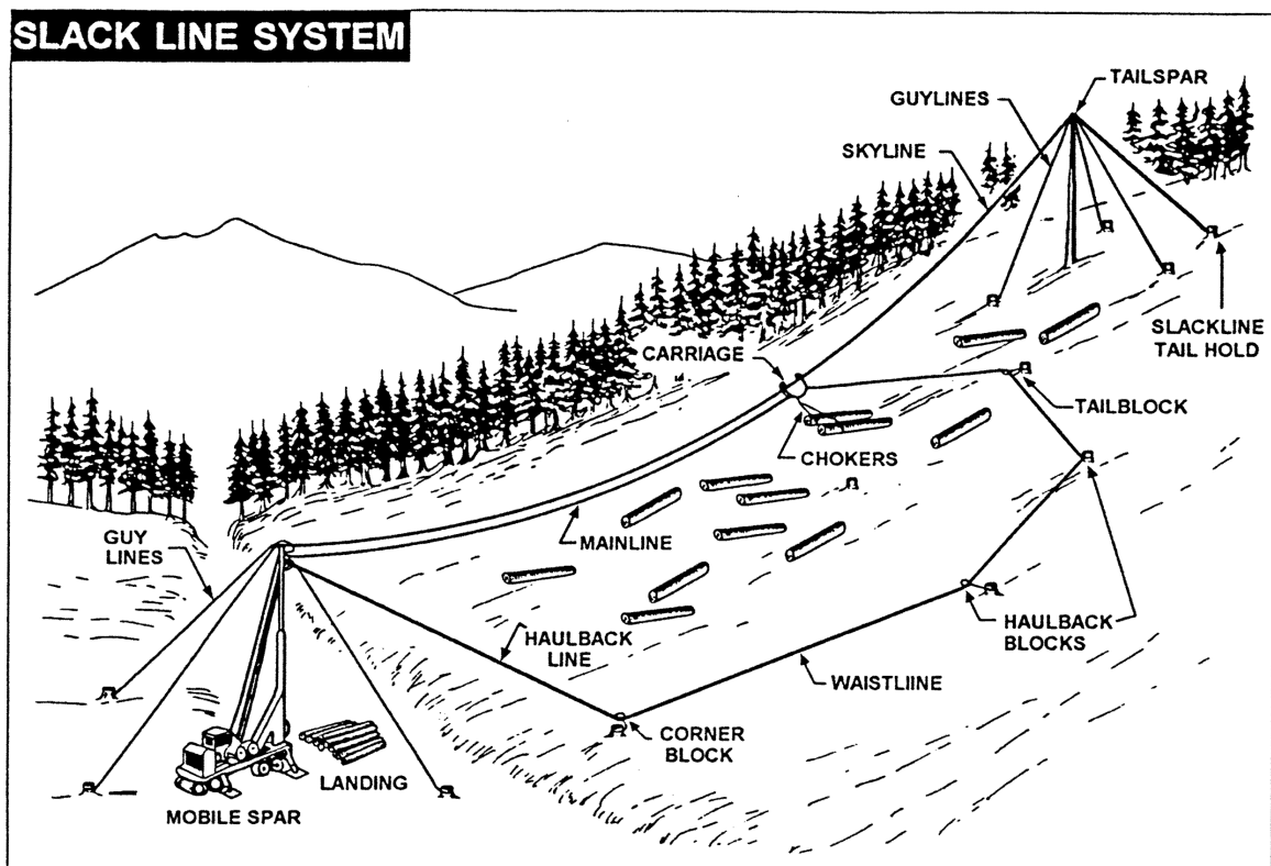
Figure 47: Slack Line System
