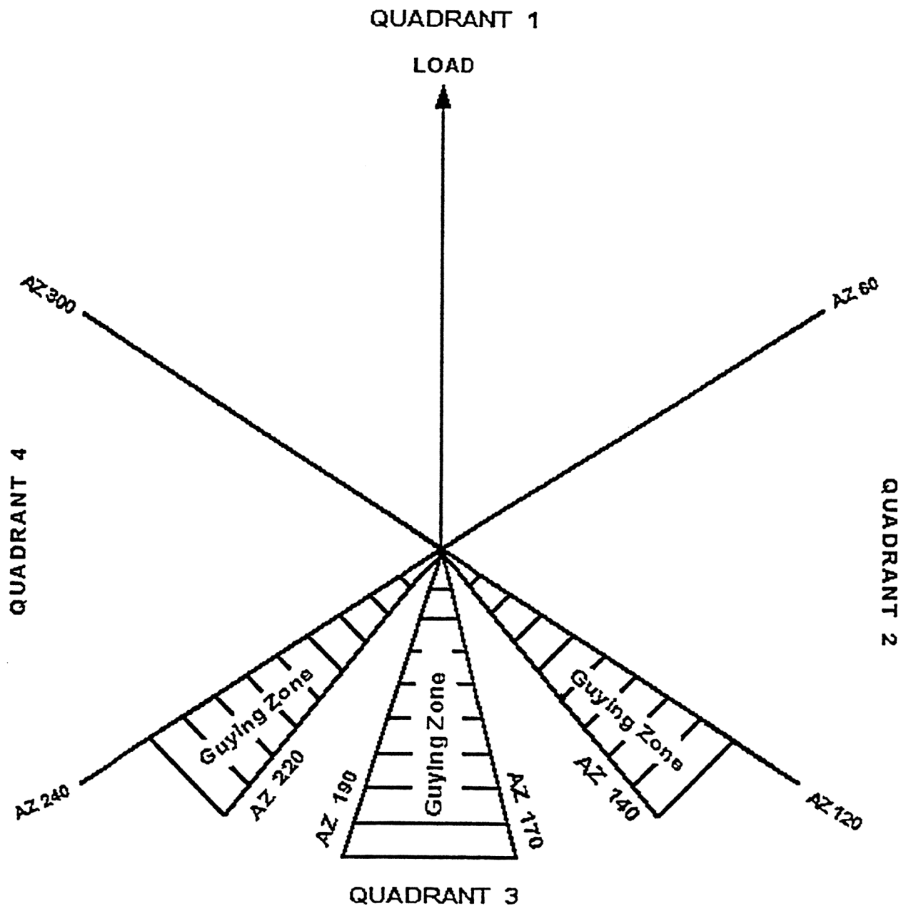
Figure 6: 3 Guyline Case
