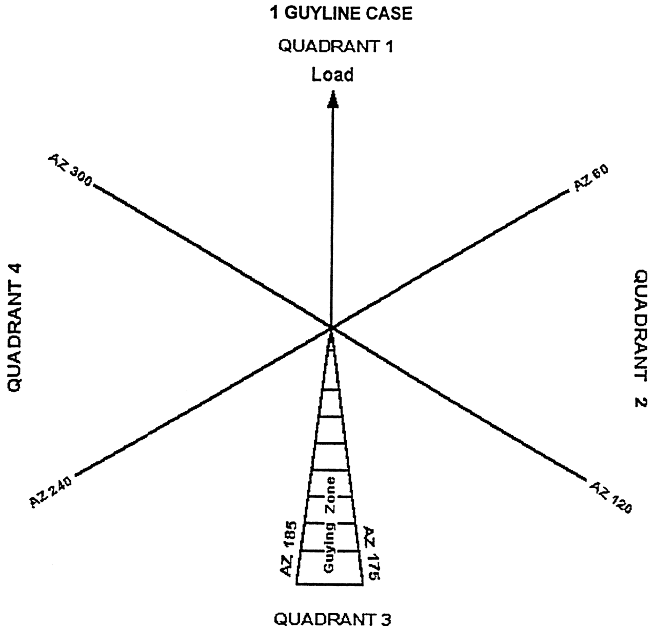
Figure 4: 1 Guyline Case
