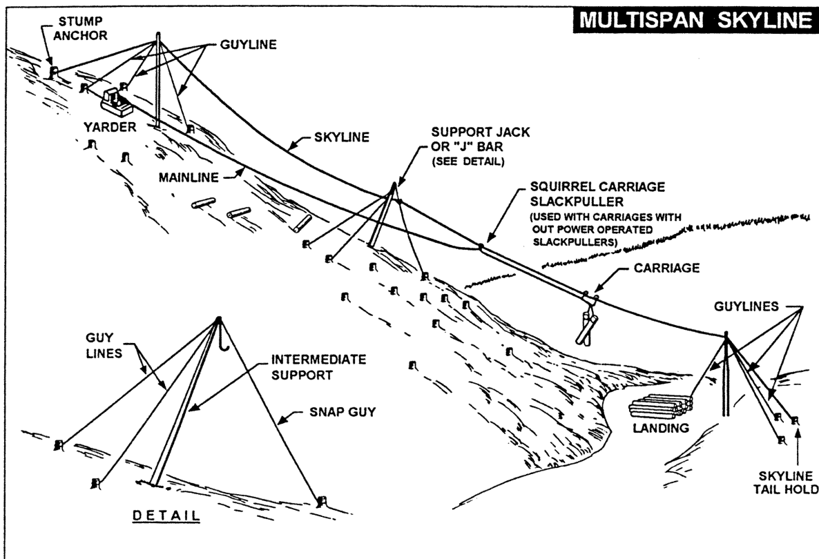
Figure 56: Multi-span Skyline
