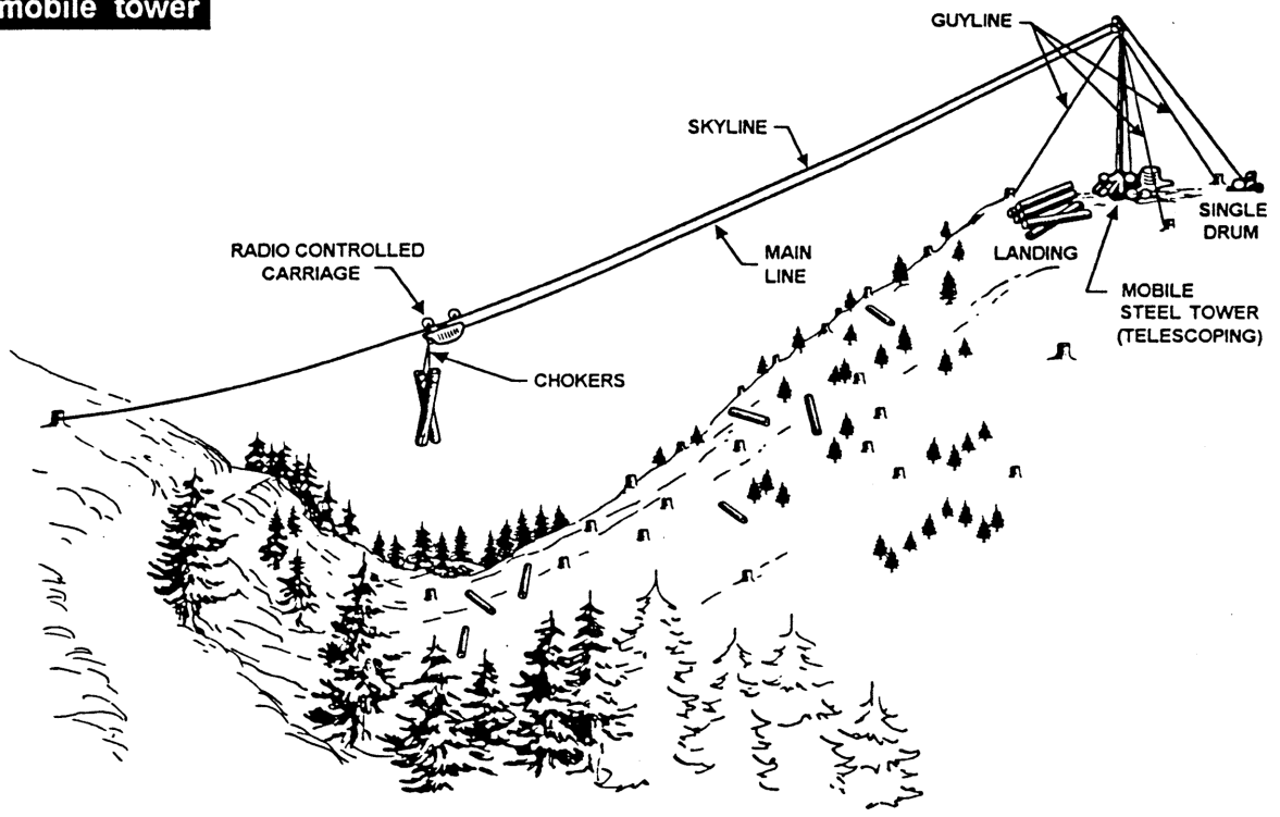
Figure 51: Standing Skyline - Radio Controlled Carriage - Mobile Tower
