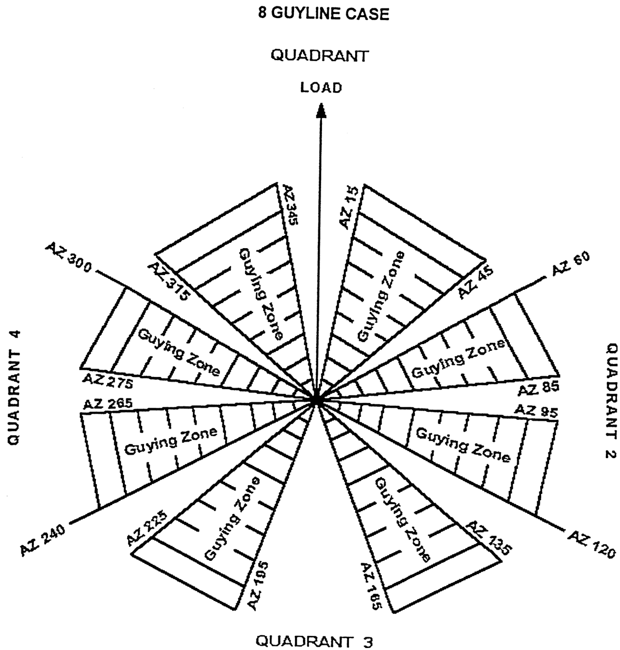
Figure 14: 8 Guyline Case
