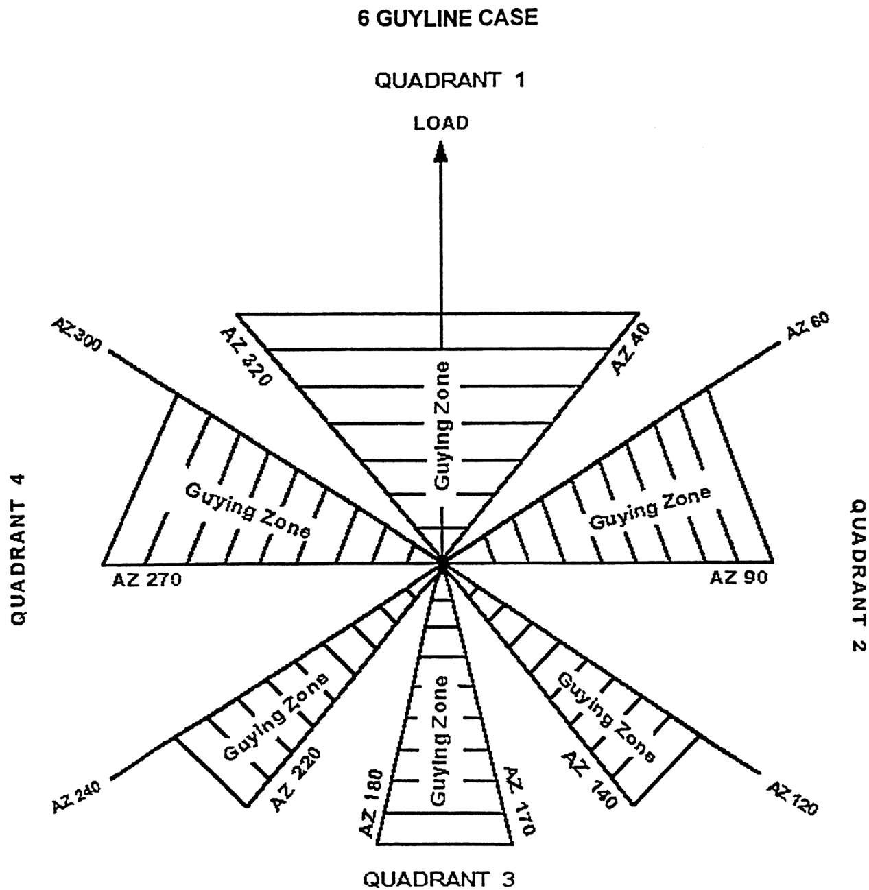
Figure 12: 6 Guyline Case (2)
