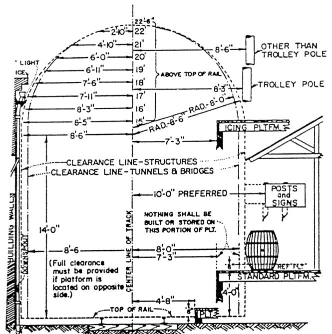
TYPICAL CLEARANCE OF STRUCTURES FROM RAILROAD TRACKS
