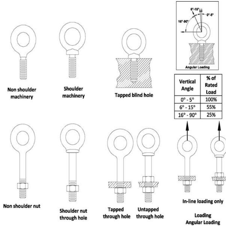
Figure 20 Eyebolts
