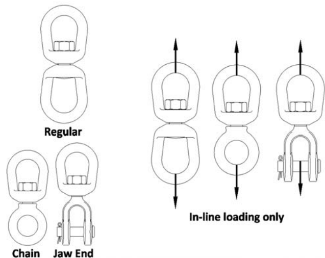
Figure 38 Swivels
