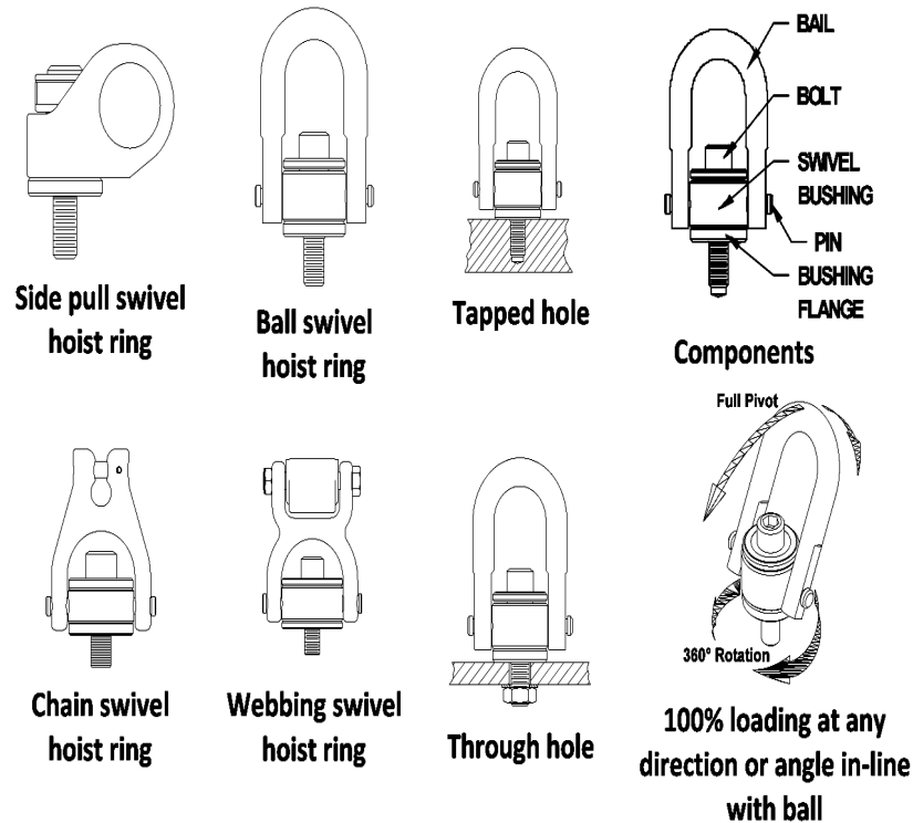
Figure 23 Swivel Hoist Rings
