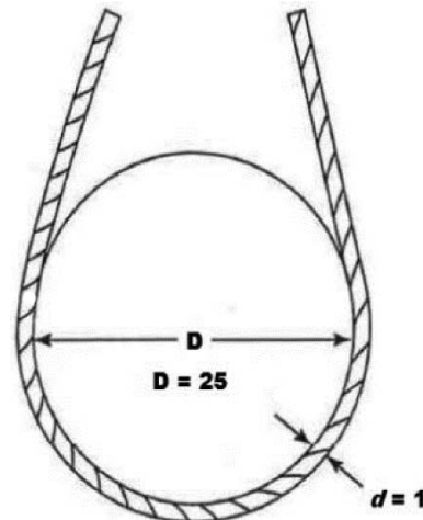
Figure 8 D/d Ratio
