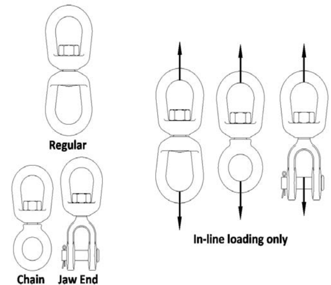
Figure 27 Swivels
