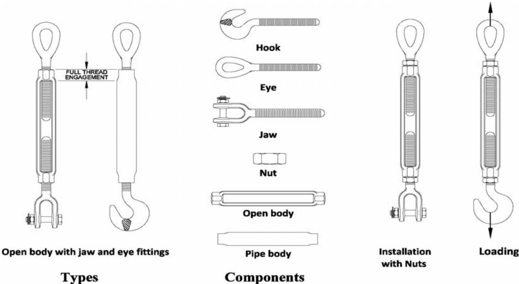
Figure 19 Turnbuckle Types
