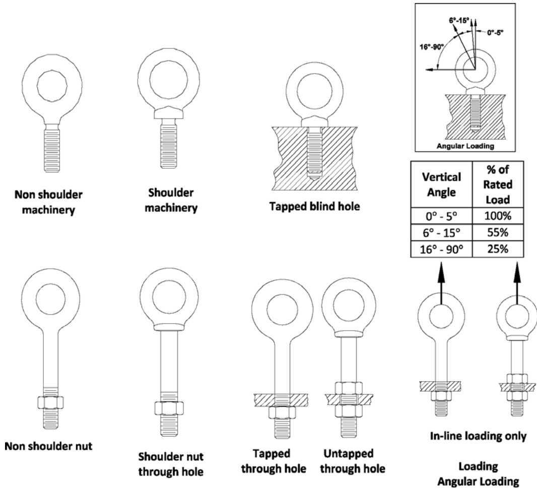
Figure 31 Eyebolts
