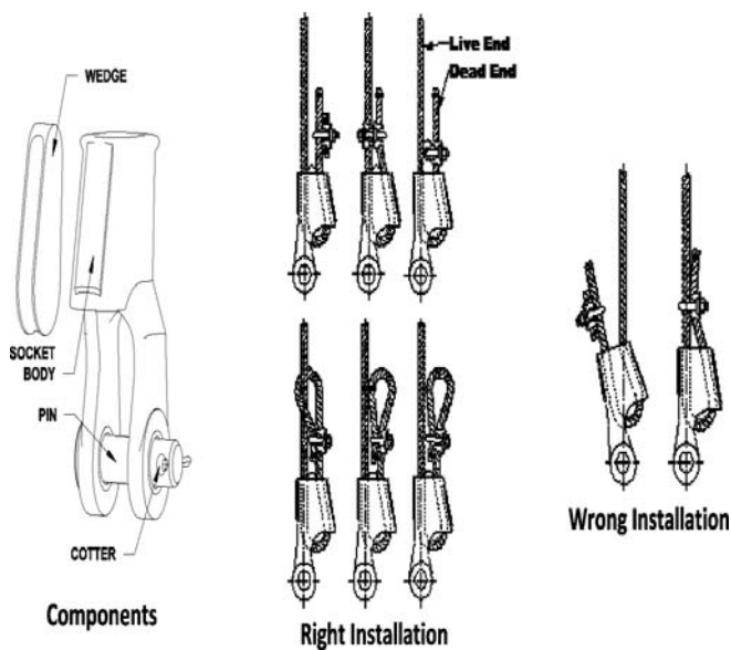
Figure 25 Wedge Sockets
