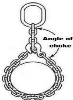
Figure 2 Single-Leg Choker Hitch
