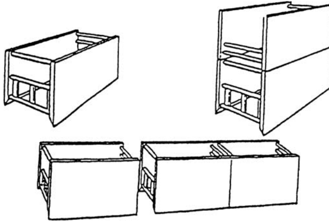
Figure N-26, Trench Shields
