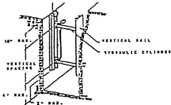
Figure N-23, Aluminum Hydraulic Shoring
