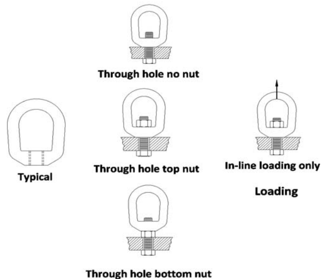
Figure 21 Eye Nuts
