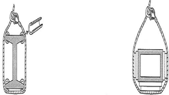
Figure 3 Softeners
