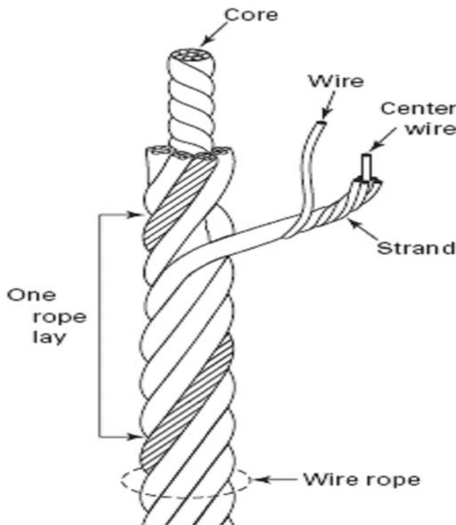
Figure 1 - Wire Rope
