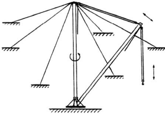
Guyed Derrick
