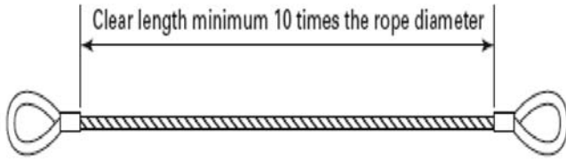
Figure 4 Minimum Sling Length For rope with 6x19 and 6x36 classification or Cable Laid Slings
