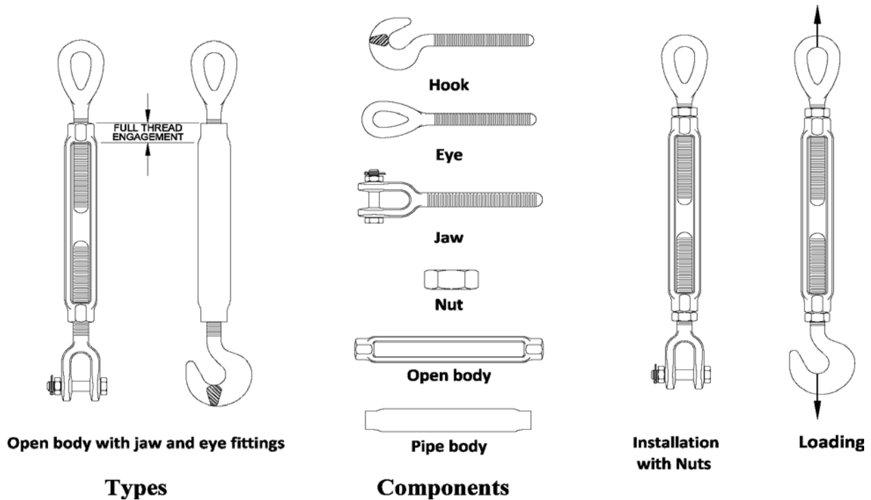
Figure 30 Turnbuckle Types
