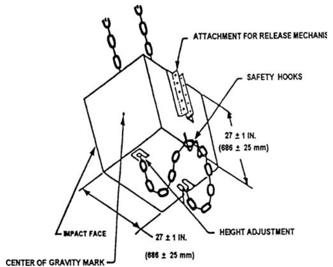
FIGURE V-22 Pendulum.
