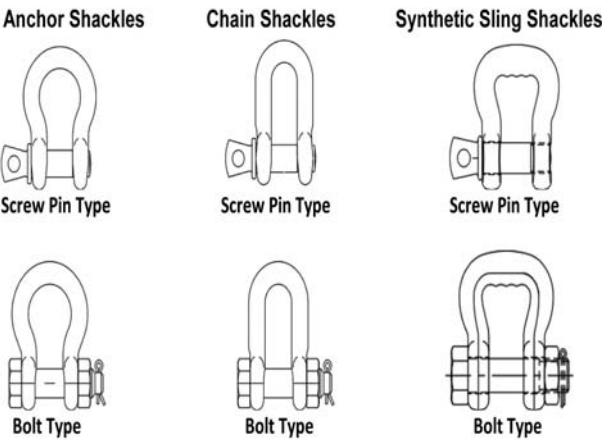
Figure 18 Shackle Types
