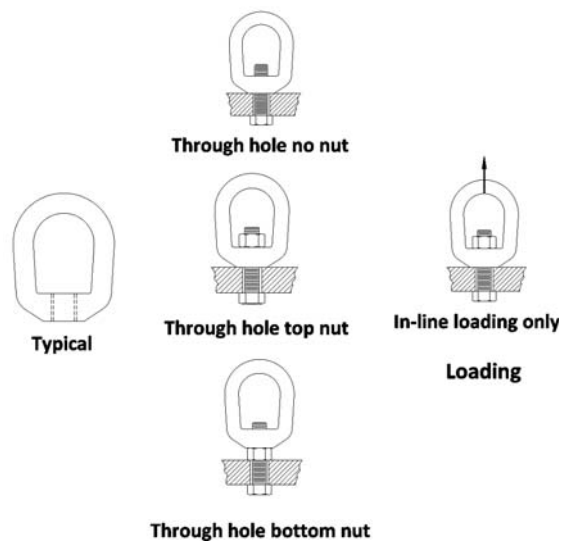
Figure 32 Eye Nuts
