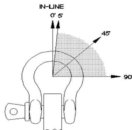
Figure 17 Side Loading
