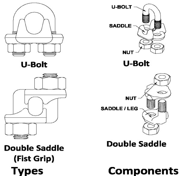
Figure 24 Wire Rope Clips
