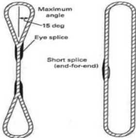
Figure 12 Synthetic Fiber Rope Slings
