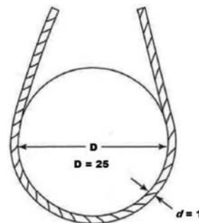
Figure 19 D/d Ratio
