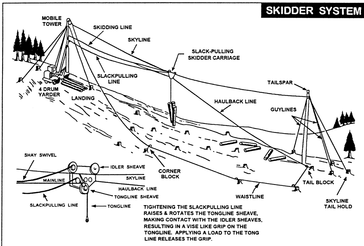
Figure 48: Skidder System
