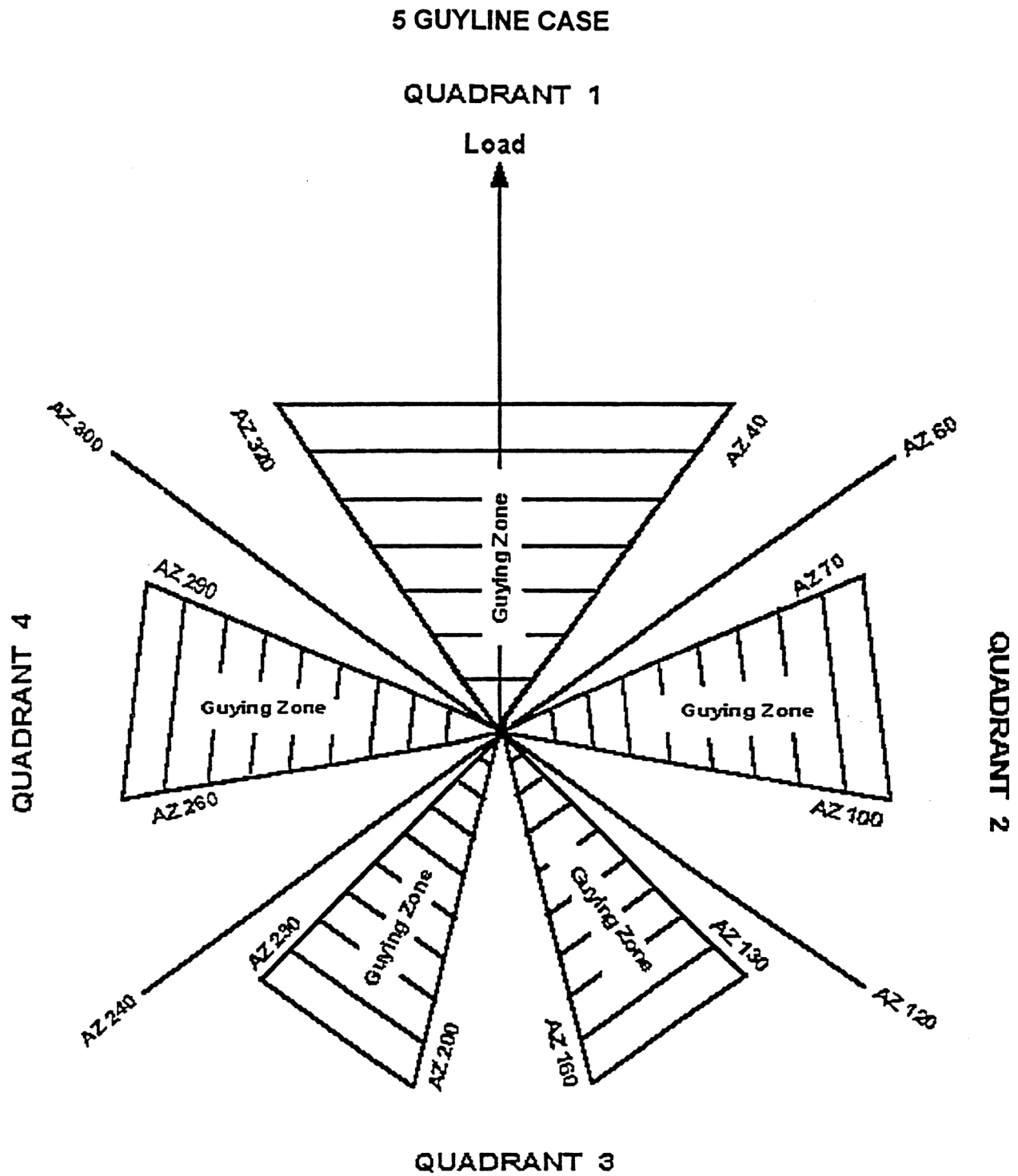
Figure 9: 5 Guyline Case
