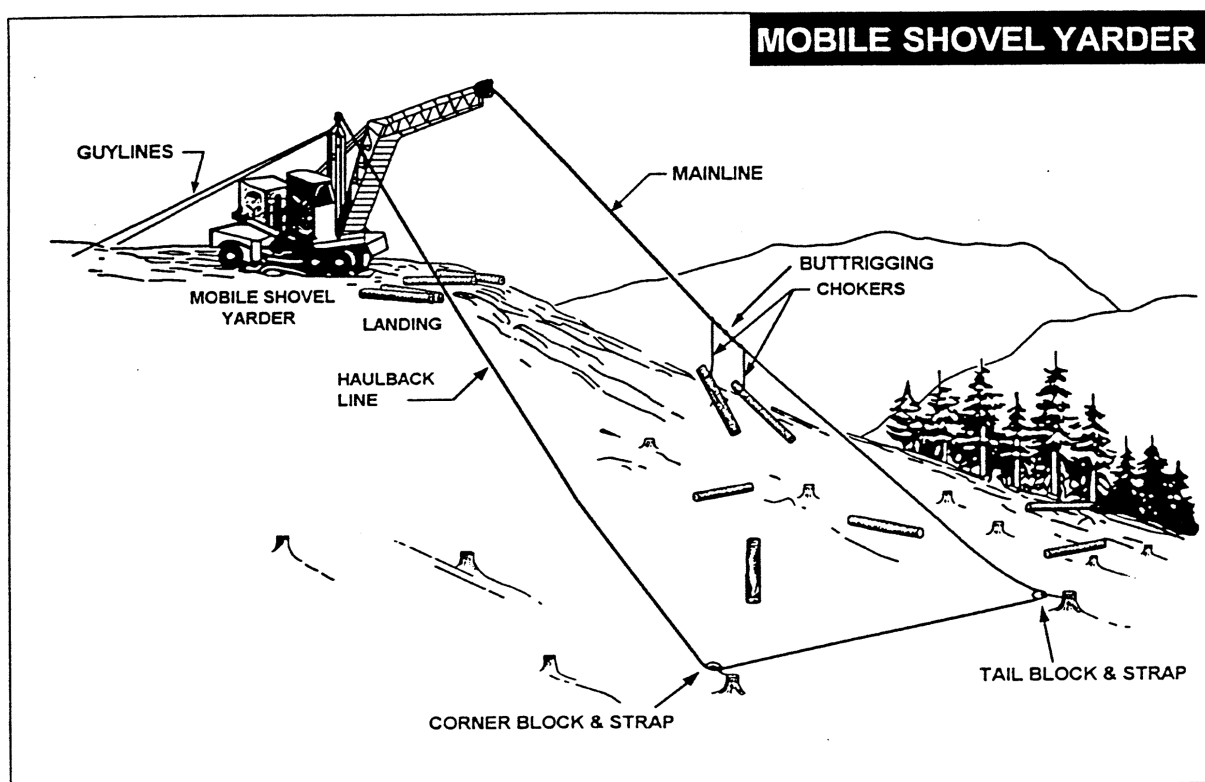
Figure 44: Mobile Shovel Yarder
