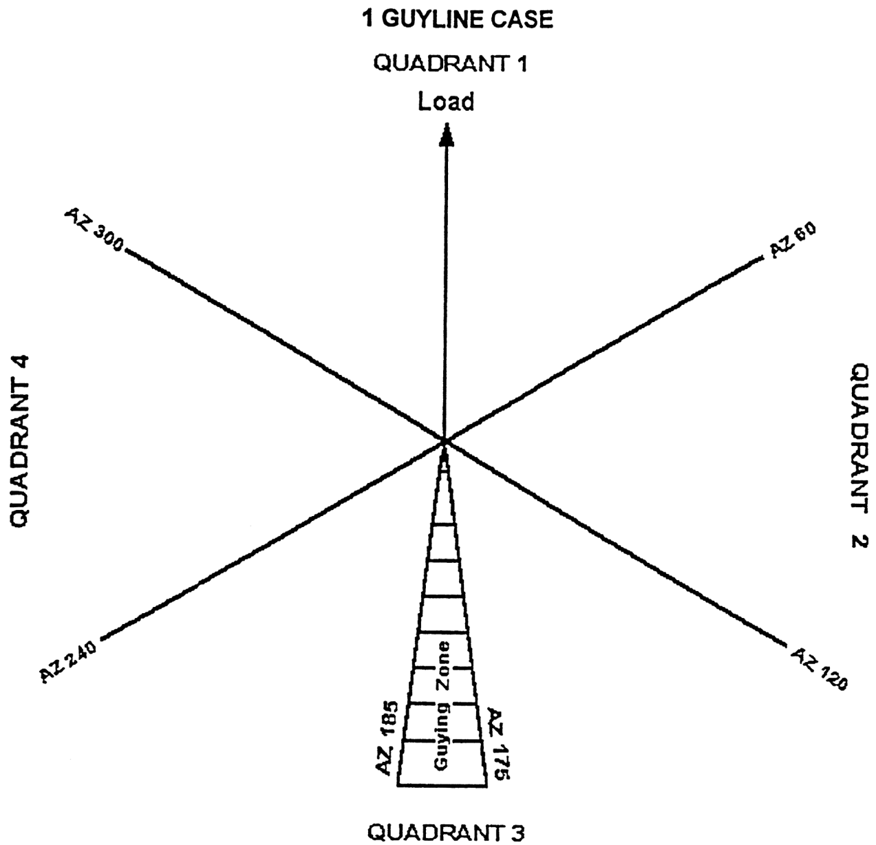
Figure 4: 1 Guyline Case
