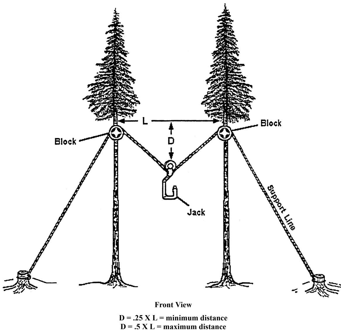
Figure 22: Double Tree Intermediate Support System
