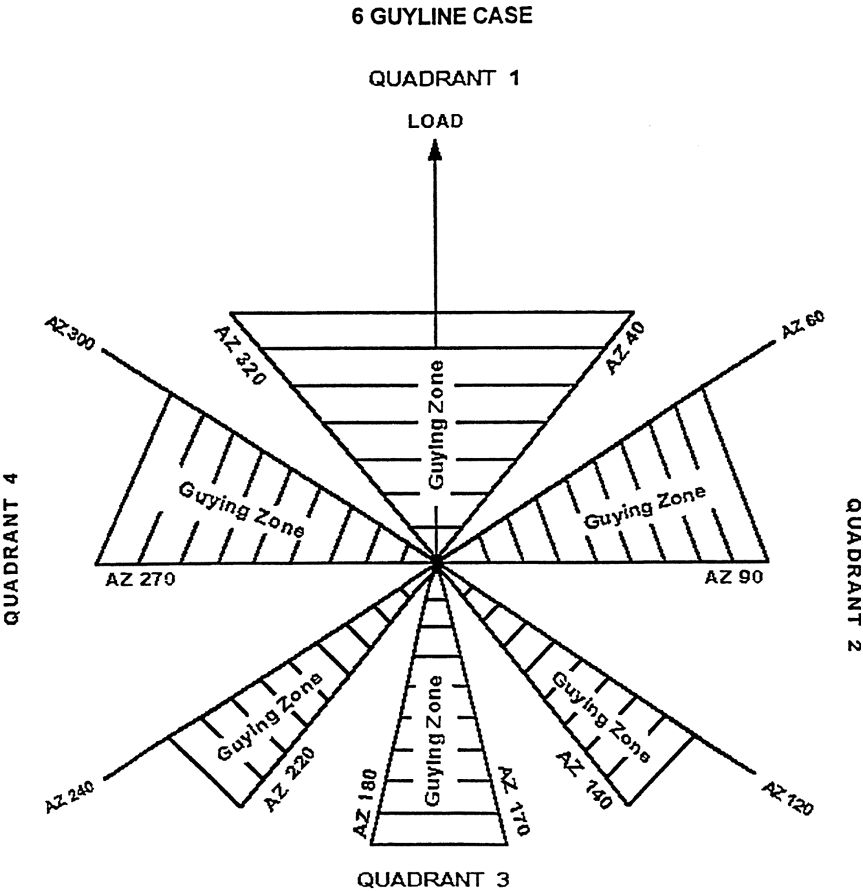
Figure 12: 6 Guyline Case (2)
