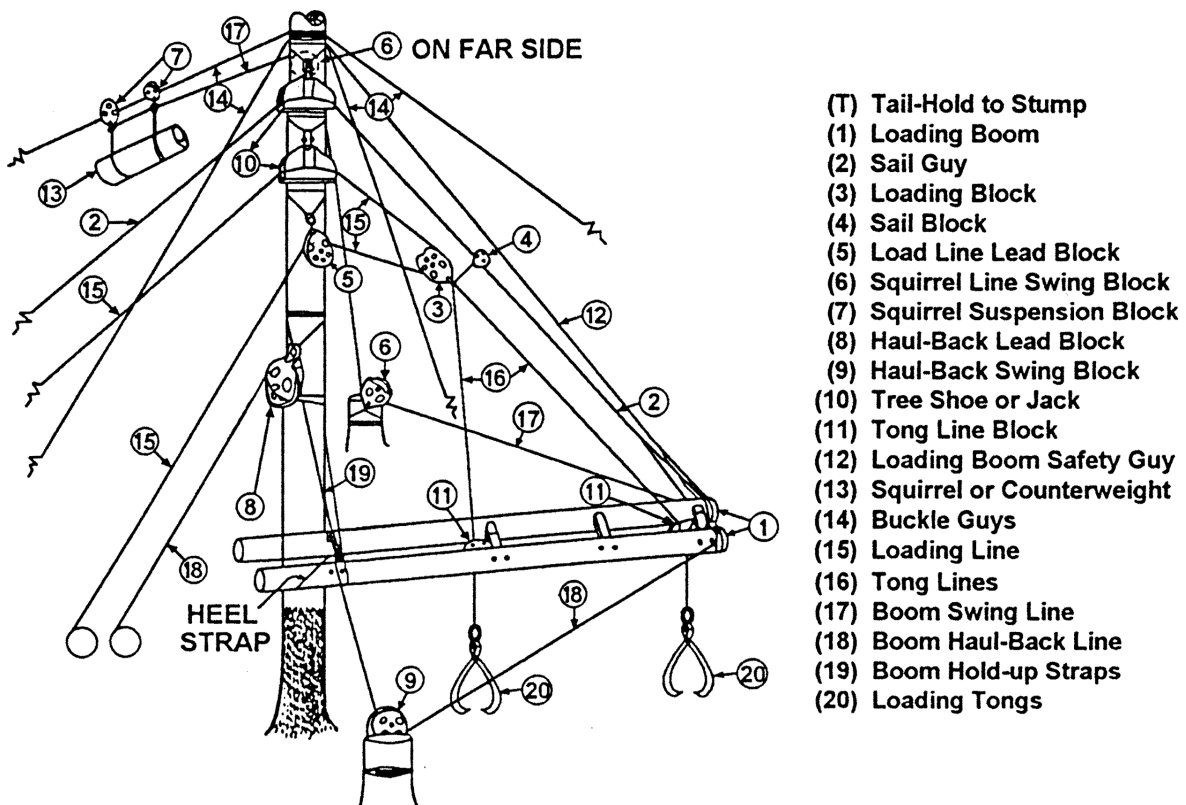
Figure 64: Hayrack Boom Loading
