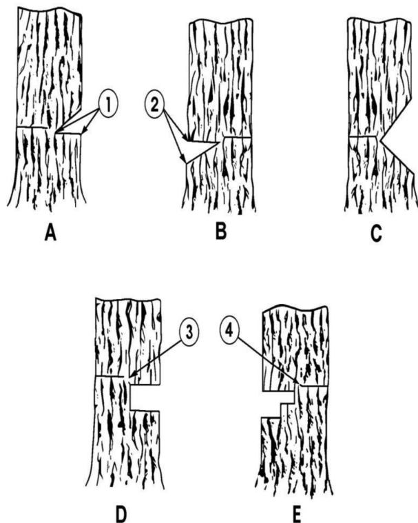
FIGURE 2: UNDERCUTS
