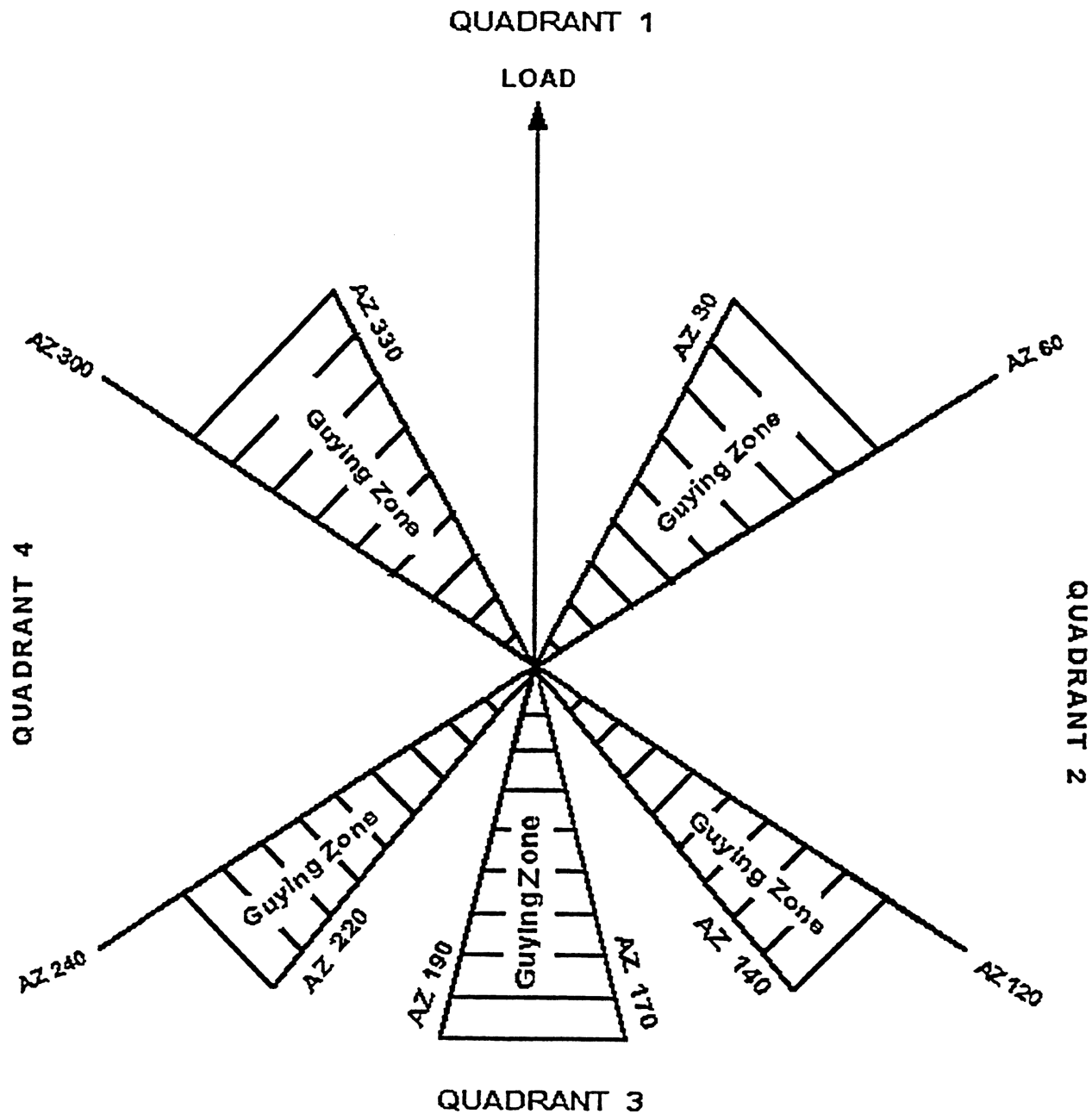
Figure 10: 5 Guyline Case (2)
