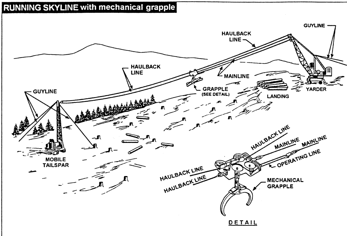
Figure 55: Running Skyline with Mechanical Grapple
