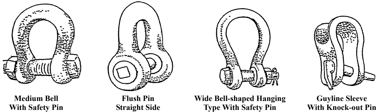
Figure 2-2: Shackles
