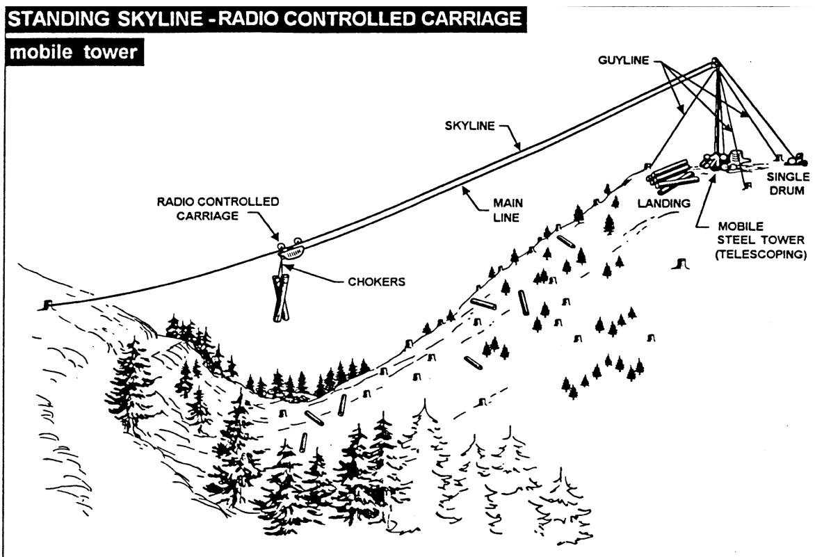
Figure 51: Standing Skyline - Radio Controlled Carriage - Mobile Tower
