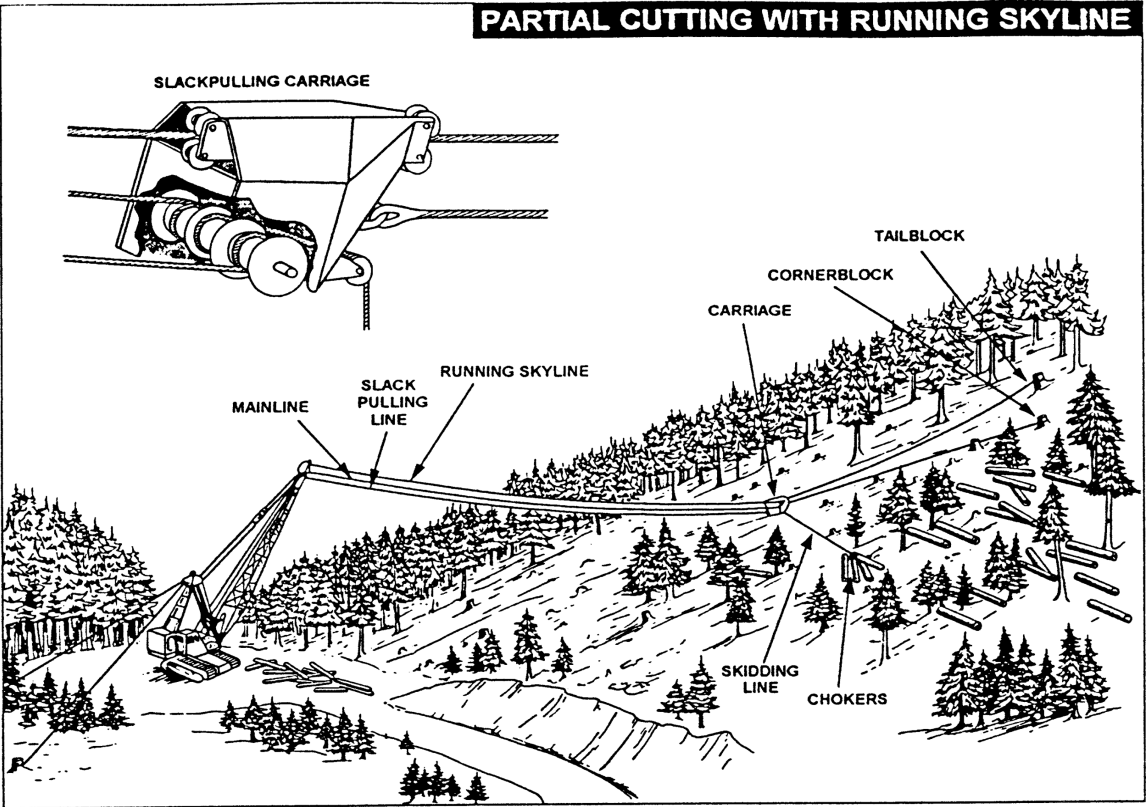
Figure 53: Partial Cutting with Running Skyline
