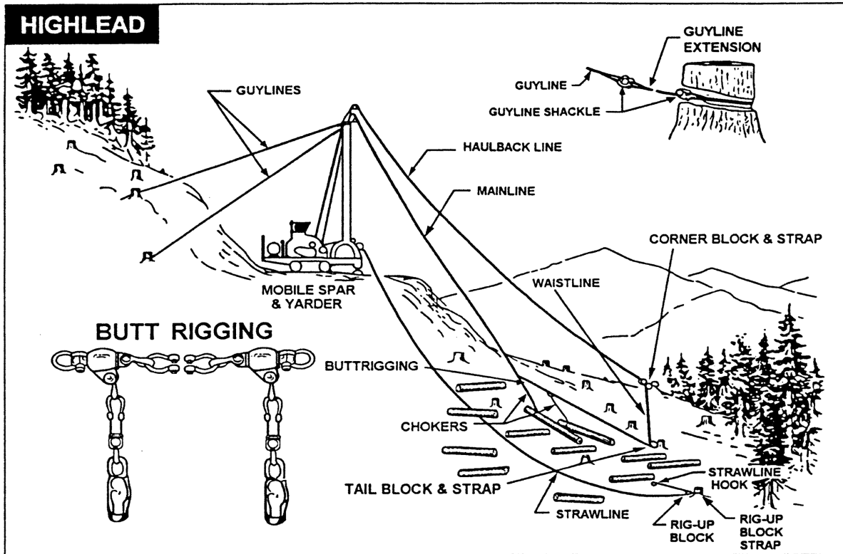
Figure 45: Highlead
