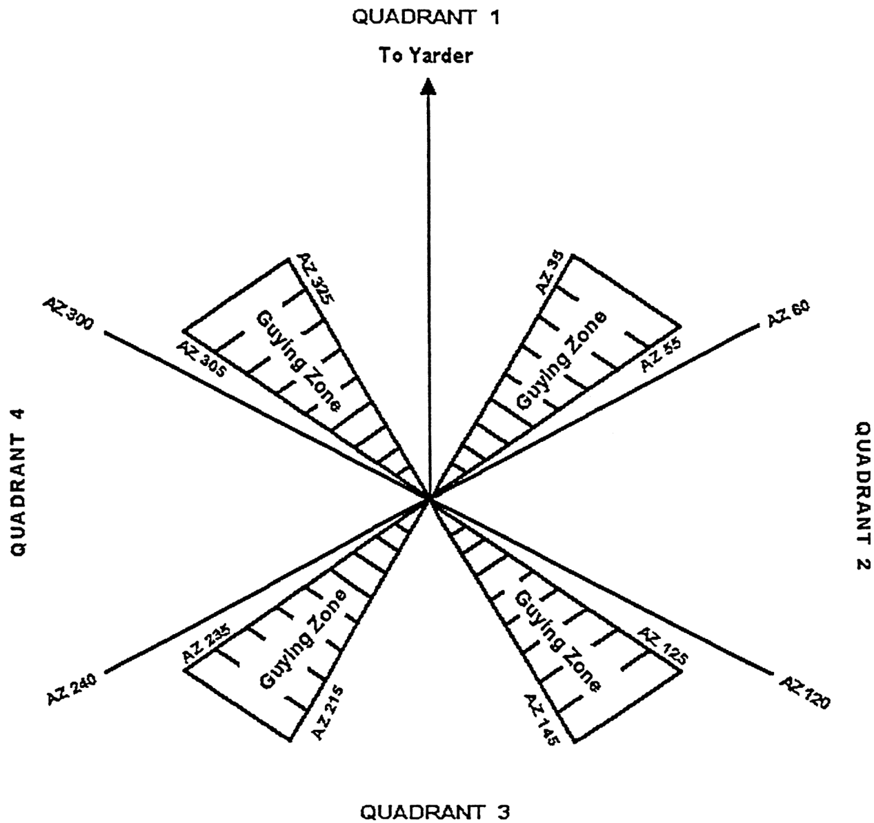
Figure 19: 4 Guyline Case - Tail/Lift Tree Gying
