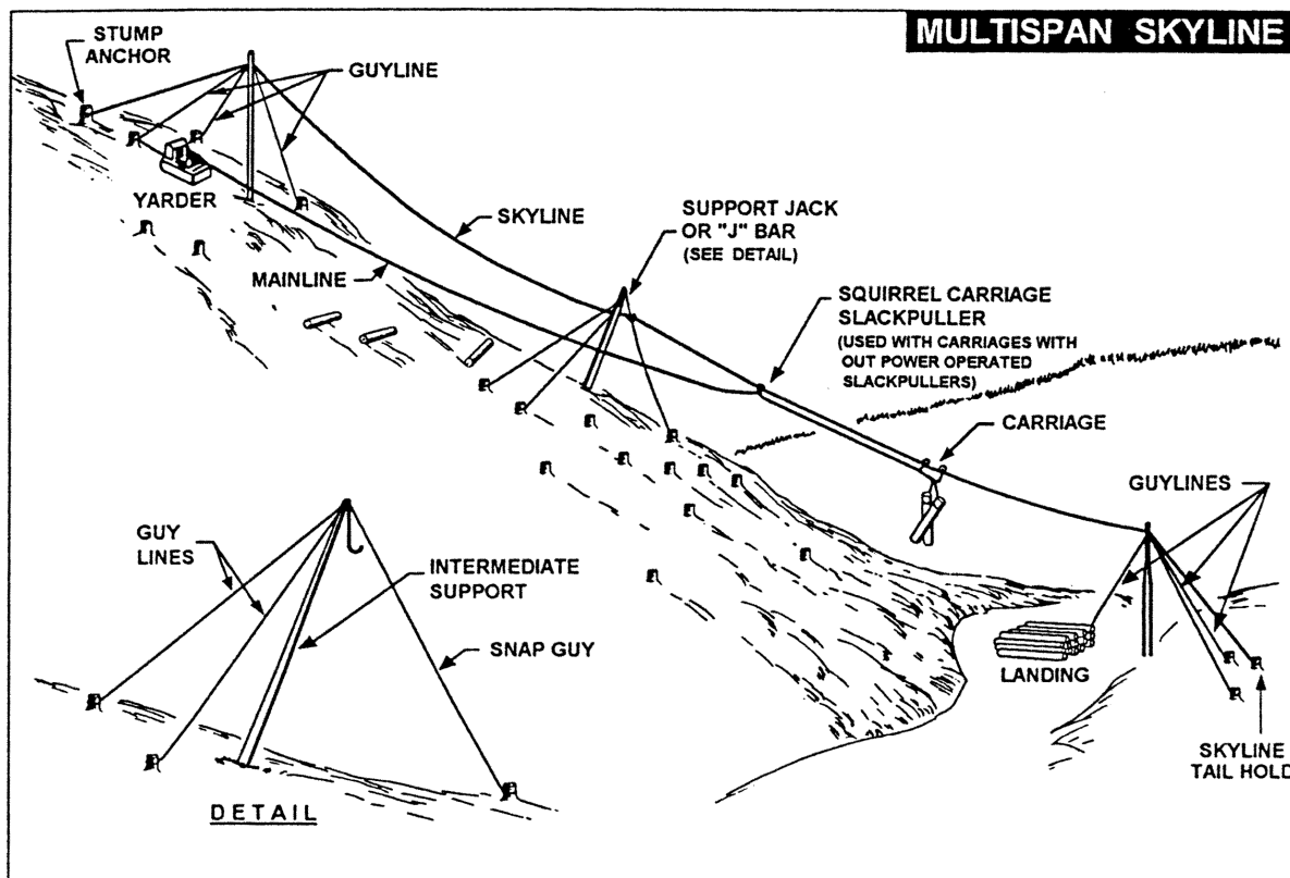
Figure 56: Multi-span Skyline
