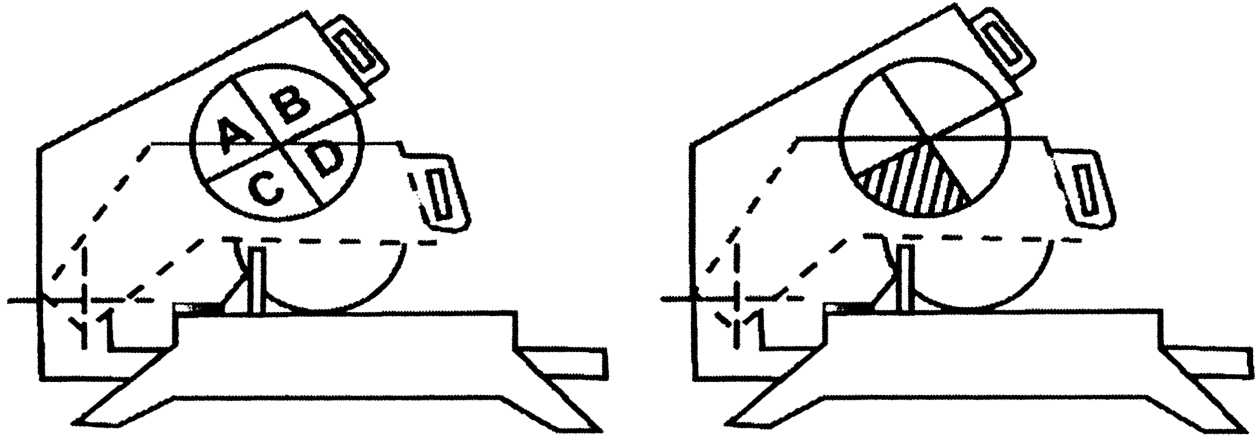
Illustration 480-1 Miter Saw Guarding
