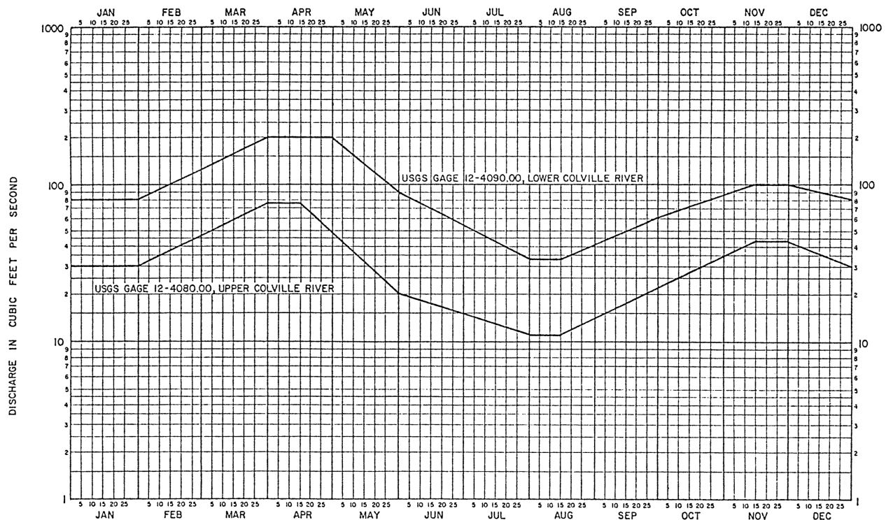
Figure 1 BASE FLOW HYDROGRAPH FOR SELECTED STATIONS
