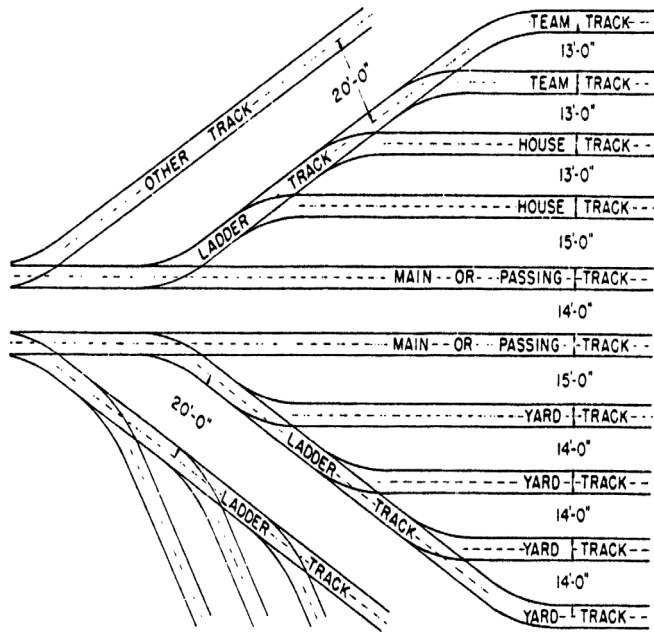
TYPICAL TRACK SPACING
