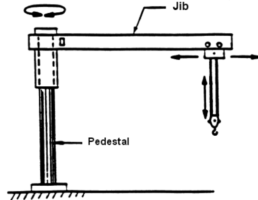
Pedestal-Jib Crane
