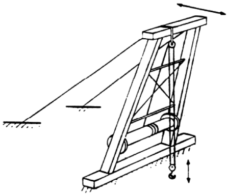
Breast Derrick
