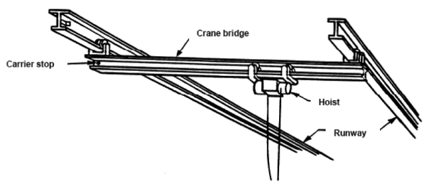
Underhung Bridge/Underhung Trolley
