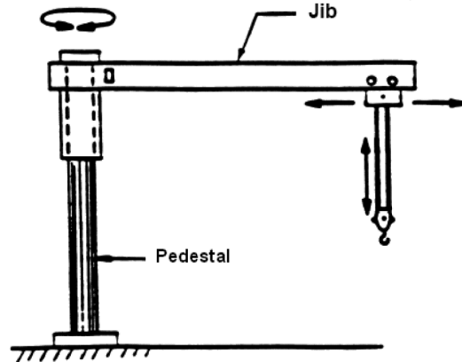
Pedestal-Jib Crane
