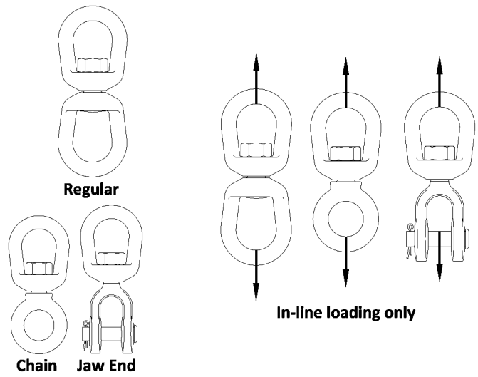
Figure 38 Swivels
