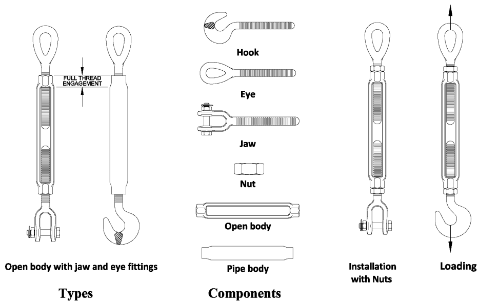
Figure 19 Turnbuckle Types
