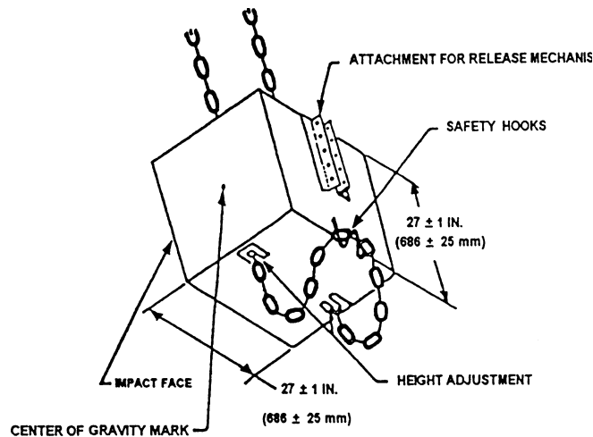
FIGURE V-22 Pendulum.
