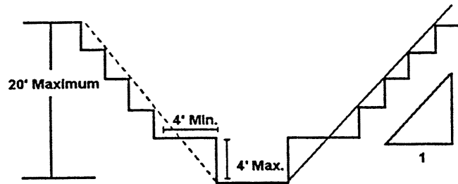
Figure N-9 Slope Configurations for Type B Soil
