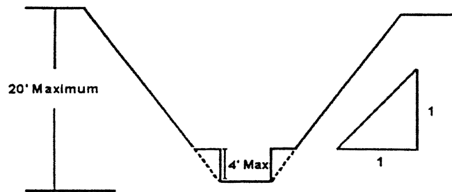
Figure N-8 Slope Configurations for Type B Soil
