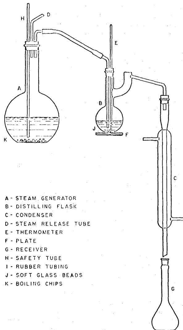
Figure 1 - Apparatus for distillation of fluoride.
