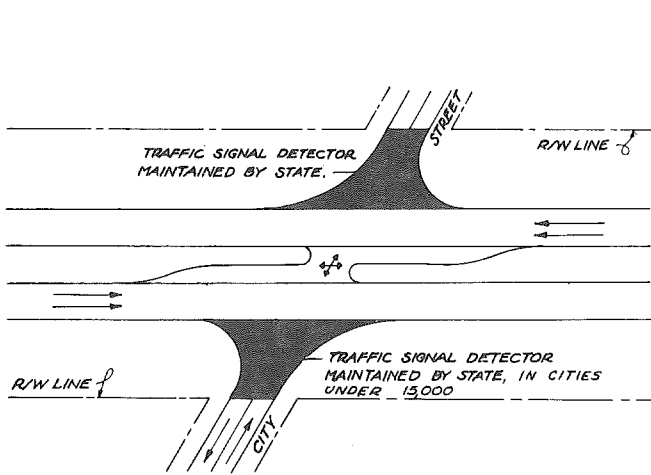
CHANNELIZED INTERSECTION NEW STATE HIGHWAY
