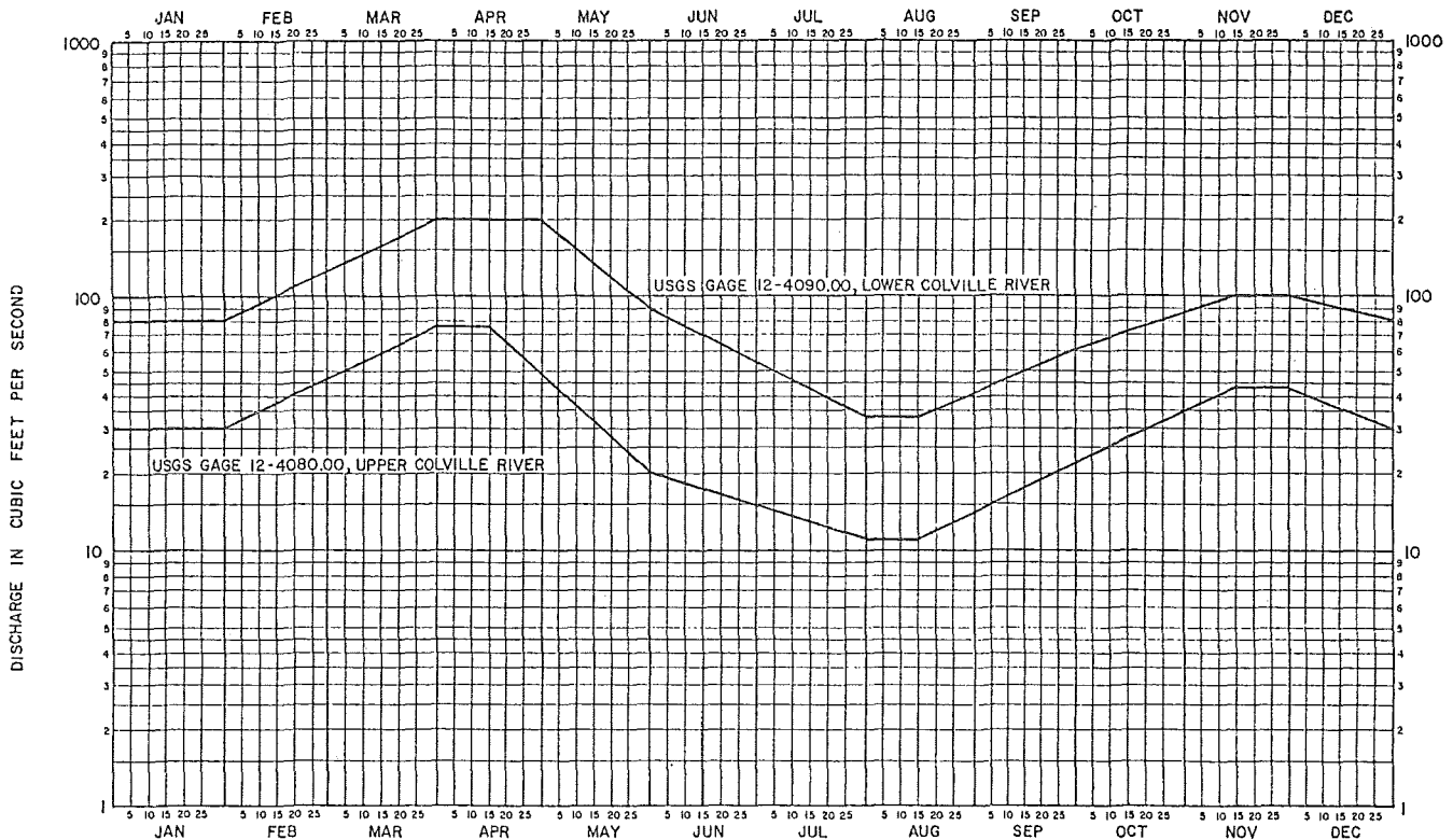
BASE FLOW HYDROGRAPH FOR SELECTED STATIONS
