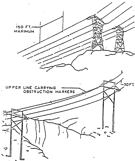
(12) Marking power lines, cables and similar obstructions.
