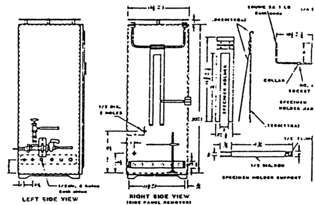
Figure L-3 - Vertical flame resistance textile apparatus, views and details. All given dimensions are in inches. System International (S.I.) unit: 1 inch = 2.54 cm.
