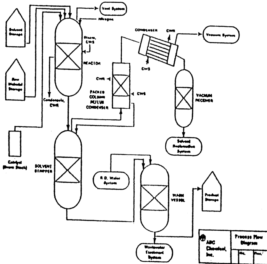
EXAMPLE OF A PROCESS FLOW DIAGRAM
