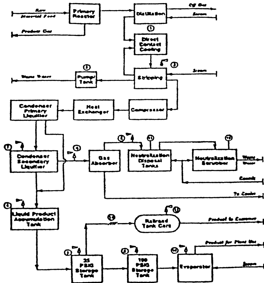
EXAMPLE OF A BLOCK FLOW DIAGRAM
