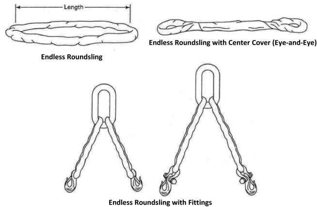
Figure 15 Synthetic Roundslings
